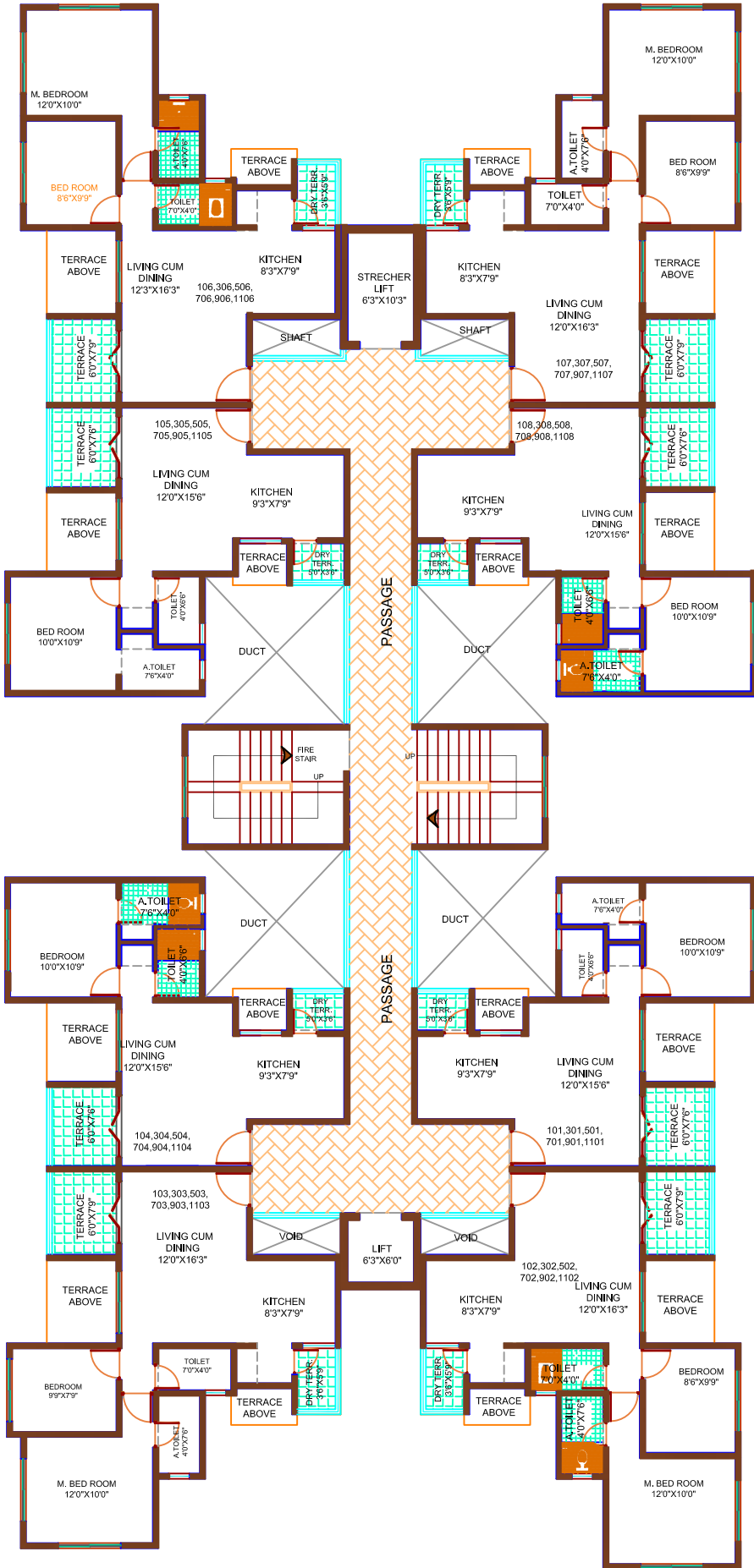
1ST/3RD/5TH/7TH/9TH/11TH FLOOR PLAN
