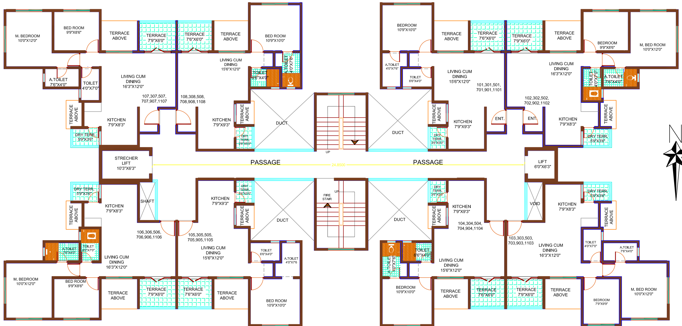
1ST/3RD/5TH/7TH/9TH/11TH FLOOR PLAN
